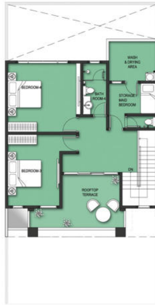
3RD FLOOR
